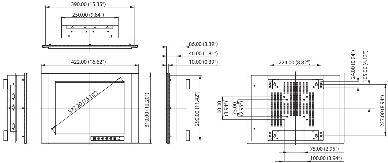
Panel Cut-out Dimensions: 396 x 296 mm (15.6" x 11.6")
