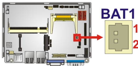
Figure 3-4: Battery Connector Location
