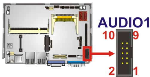
Figure 3-3: Audio Connector Location
