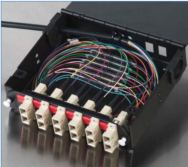
SPH-01P with SC Duplex Connector Pigtails Spliced onto FREEDM® One Cable | Photo LAN672
