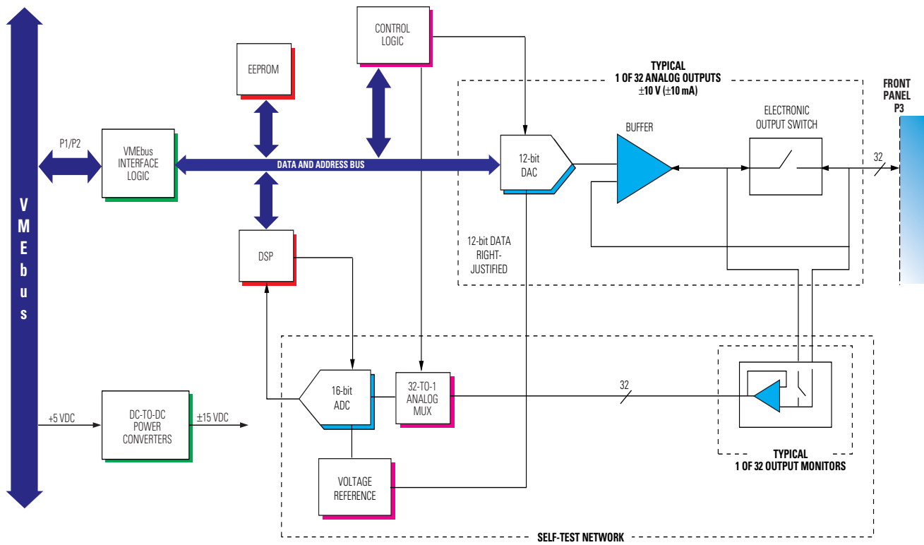
Figure 1. VMIVME-4140 Functional Block Diagram
