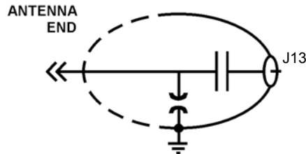
Arrester Schematic
