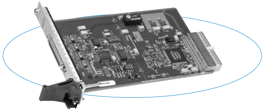
Advanced memory management techniques allow the AcPC330 to operate with minimal interruption of the A/D converter.
