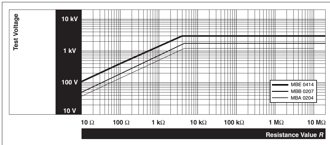
Fig.8 Pulse load rating in accordance with IEC 60115-1, 4.27; 10 μs / 700 μs; 10 pulses at 1 minute intervals; for permissible resistance change 0,5%.
