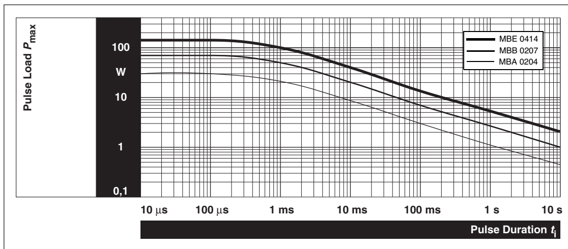
Fig.4 Maximum pulse load, single pulse; for permissible resistance change equivalent to 8000 h operation.
