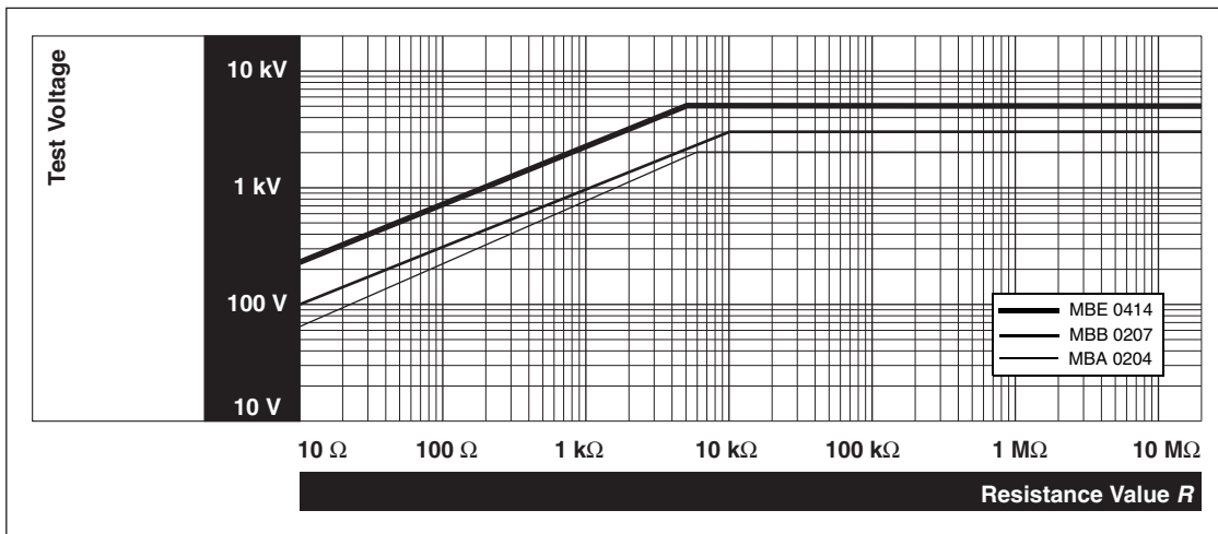
Fig.7 Pulse load rating in accordance with IEC 60115-1, 4.27; 1,2 μs / 50 μs; 5 pulses at 12 s intervals; for permissible resistance change 0,5%.
