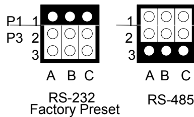
Figure 3-10 P1 & P3: RS-232/RS-485 Select for COM2
