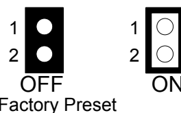
Figure 0-9 JP4: D.O.C. Memory Address Select
