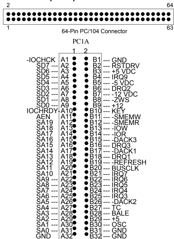
Figure PC1A: 64-Pin PC/104 Connector Bus A & B
