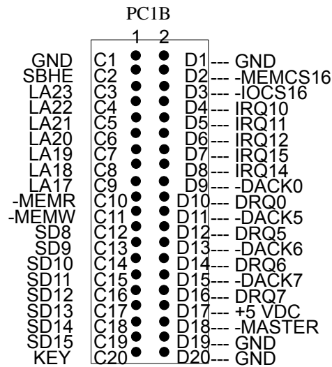
Figure PC1B: 40-Pin PC/104 Connector Bus C &amp; D
