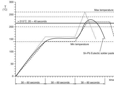
REFLOW SOLDERING
