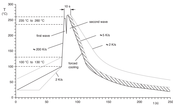
WAVE SOLDERING
