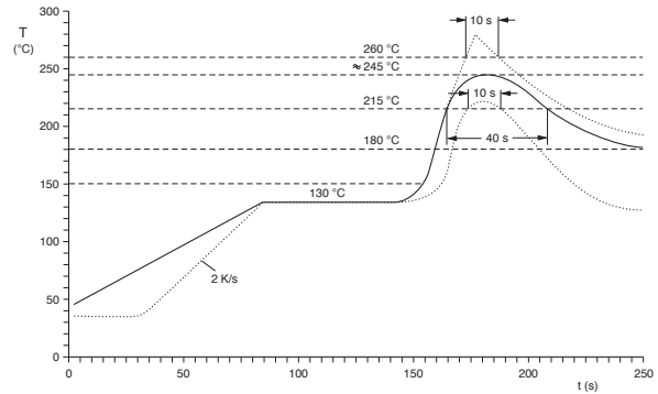
REFLOW SOLDERING
