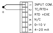
Thermocouple and Millivolt
