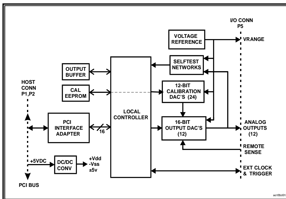
Figure 1. PMC-16AO-12 Board; Functional Organization
