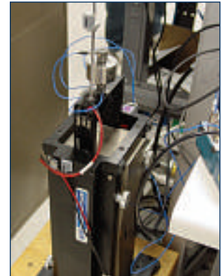
Low-frequency Accelerometer Calibrator 6" (152 mm) stroke shaker provides displacement for calibrations to 0.5 Hz
