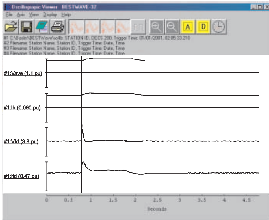
Figure 6 - BESTwave Oscillography
