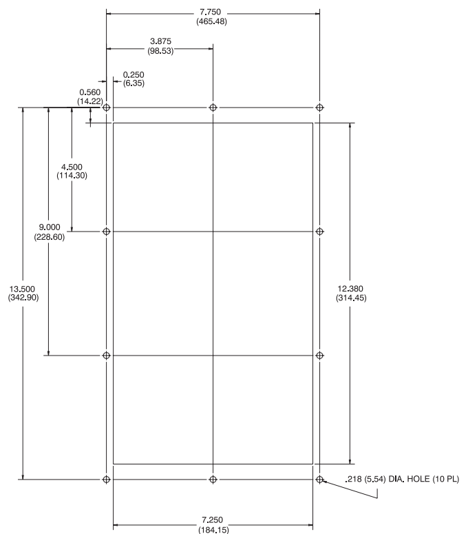
Figure 4 - Front Panel Mounting Bracket, P/N 9360107100
