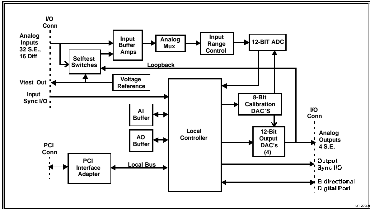
Figure 1. PCI-12AIO; Functional Organization
