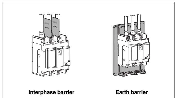
Interphase barrier
