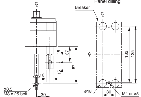
Panel drilling
