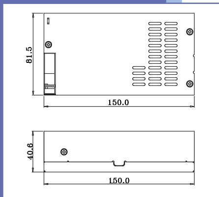
Dimensions (ACE-815T/815C)
