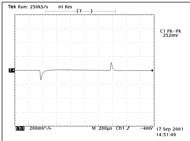
Figure 3. Output Voltage response (200mV/div) to a step-change in load current (50% - 75% - 50% of I_{max}:dl/dt=1A/\mu s . Load capacitance: 470 \mu F, 30mOhm ESR tantalum capacitor .
