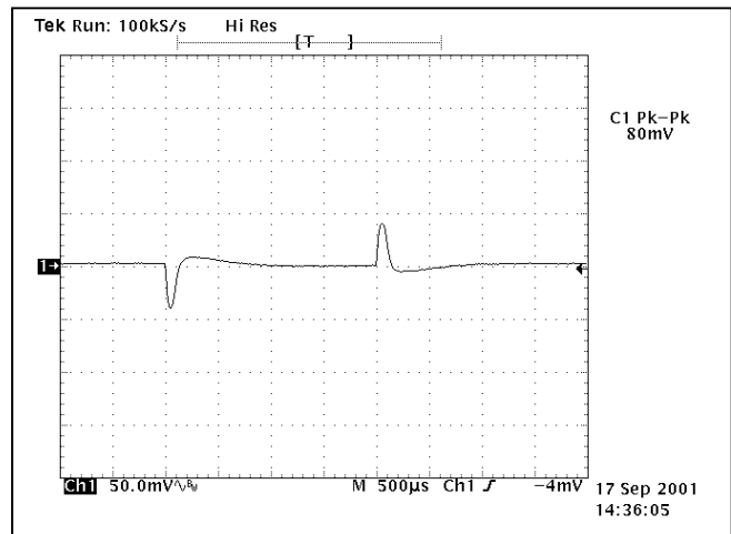
Figure 4. Output Voltage response (50mV/div) to a step-change in load current (50% - 75% - 50% of I_{max}:dl/dt=0.1A/\mu s . Load capacitance: 470 \mu F, 100mOhm ESR tantalum capacitor .
