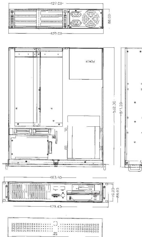
BACKPLANE VERSION
