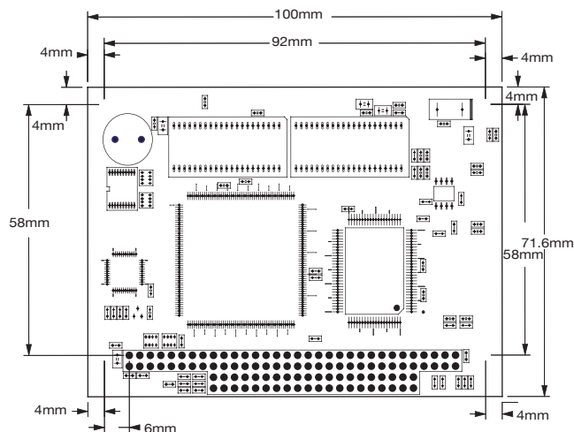
Component Side
