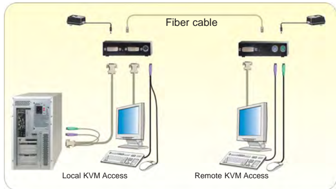
Figure 15. Typical cabling configurations
