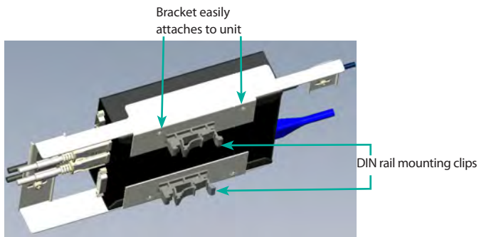
Figure 11. Div. 2 mounting bracket
