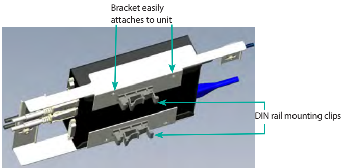
Figure 16. Div. 2 mounting bracket
