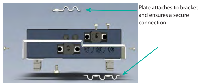
Figure 4. Div.2 mounting bracket
