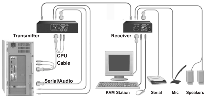
Figure 3. Cabling
