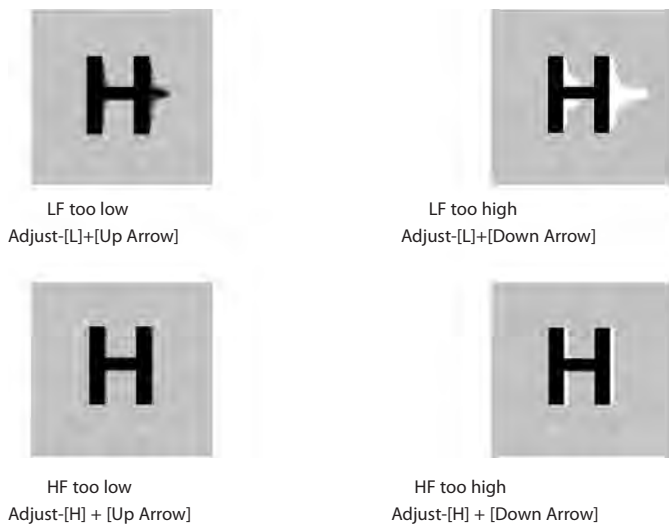
Figure 7. HF / LF adjustment guide
