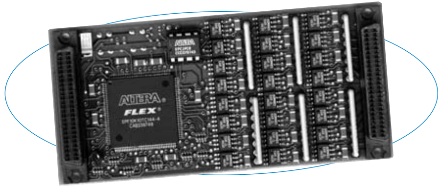
The IP409 has 24 channels with interrupts for reliable, high-speed serial or parallel data transfer across noisy environments.
