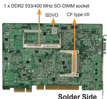
Solder Side
