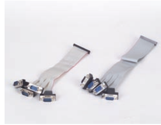
P/N 1701400181 Flat cable IDC 2 x 20-pin pitch : 2.0 mm to D-SUB (9P Female) 4 COM, L = 18 cm
