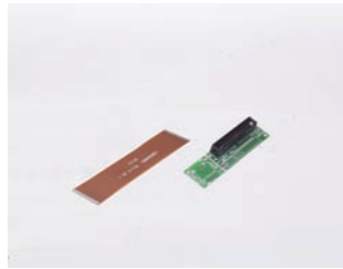
P/N 9681000044E Purch 26-34-pin FDD cable converter (+5 V)
