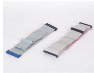
P/N 1701400452 Flat cable 2 x 20-pin (blue) to 2 x 20-pin (gray) to 2 x 20-pin (black), L = 45 cm
