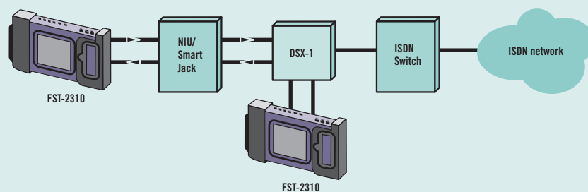
figure 7 Perform ISDN terminal emulation as well as monitor ISDN links from DS1, DS3 and STS-1 circuits
