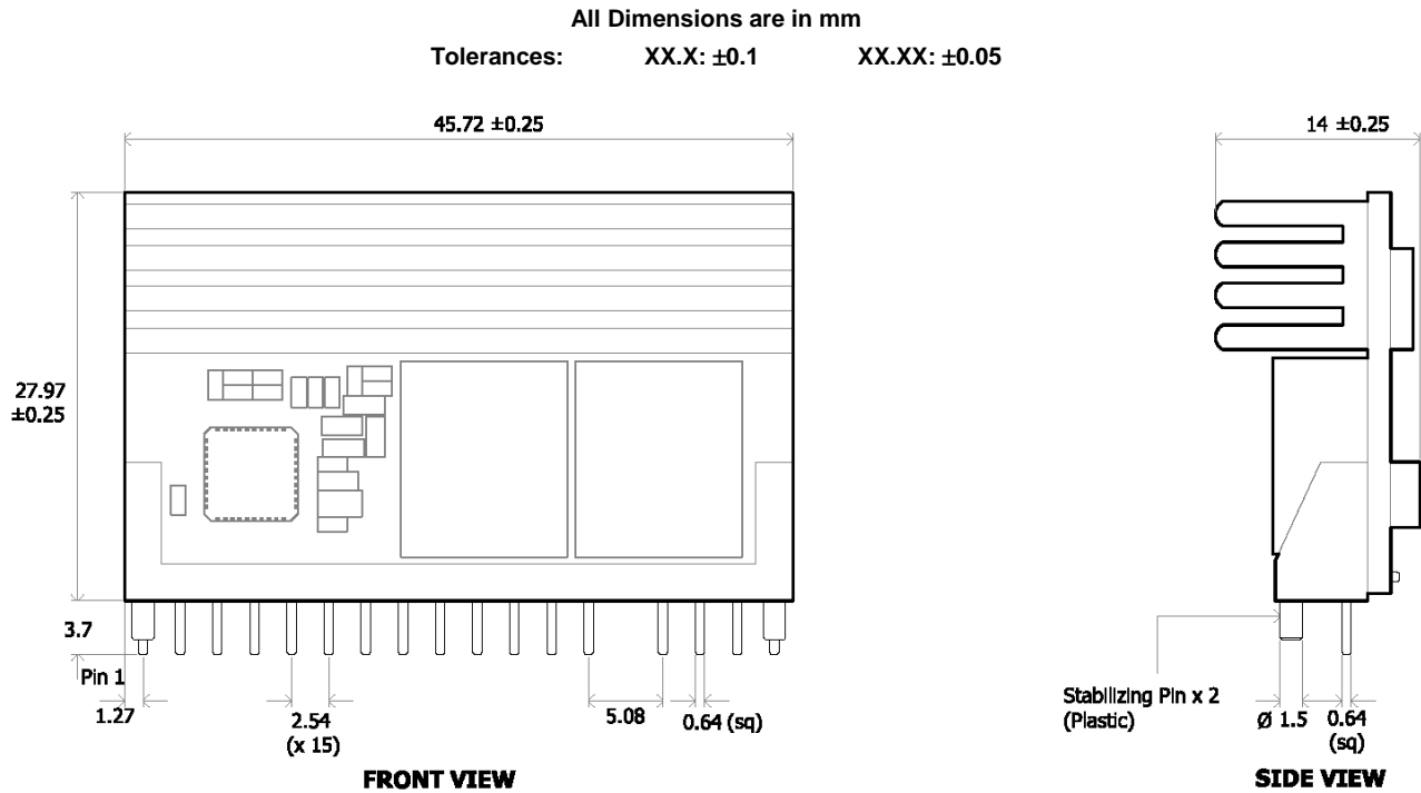
Figure 47. Mechanical Drawing
