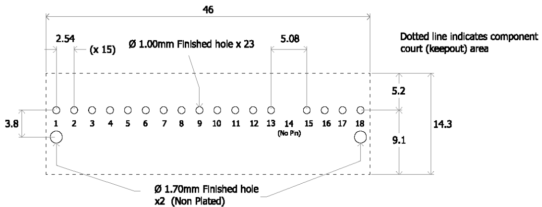
Figure 48. Recommended Footprint – Top View
