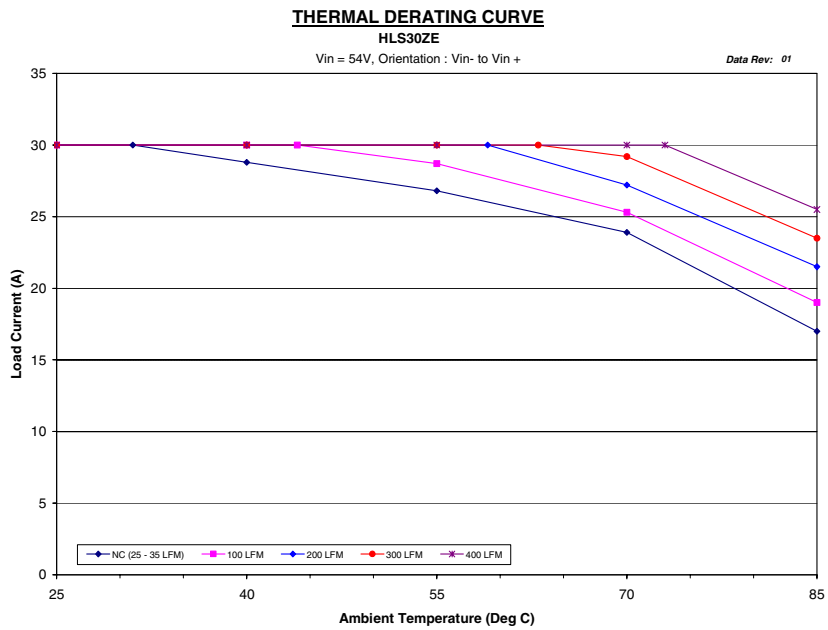
Figure 10. HLS30ZE (3.3V) Derating Curves
