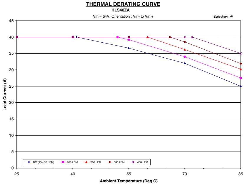
Figure 11. HLS40ZA (1.5V) Derating Curves
