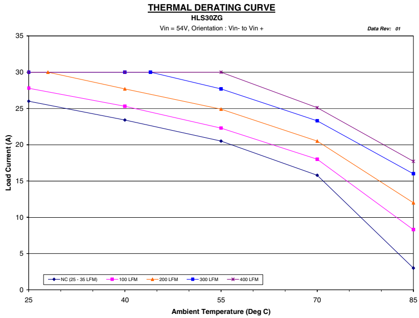
Figure 9. HLS30ZG (5V) Derating Curves
