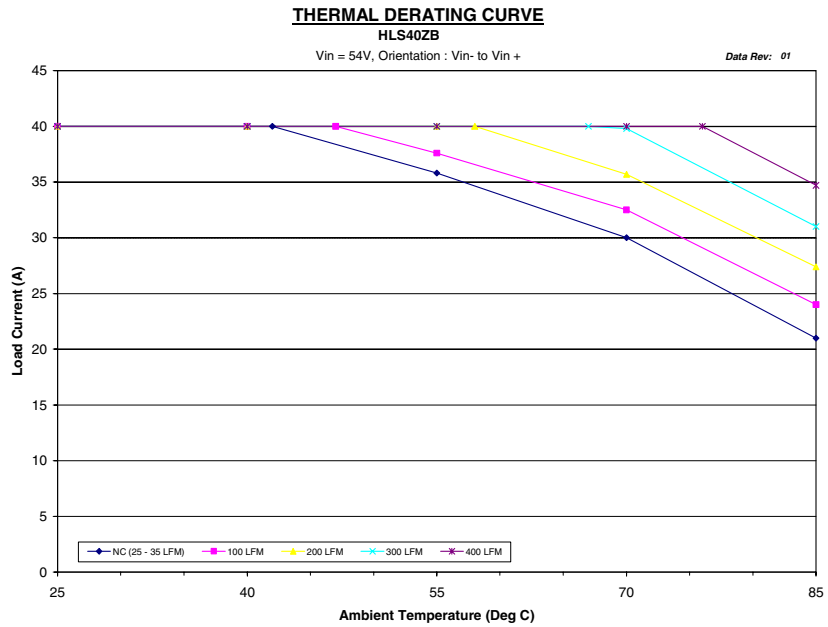
Figure 12. HLS40ZB (1.8V) Derating Curves
