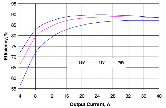
Figure 5. HLS40ZB (1.8V) Efficiency vs. Output Load
