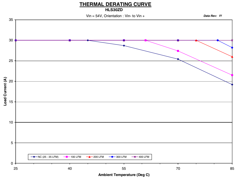
Figure 13. HLS30ZD (2.5V) Derating Curves
