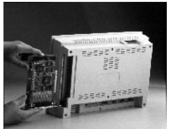
The PPC-140/120's PCI/ISA expansion slot
