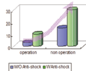
Unit: G Shock Test
