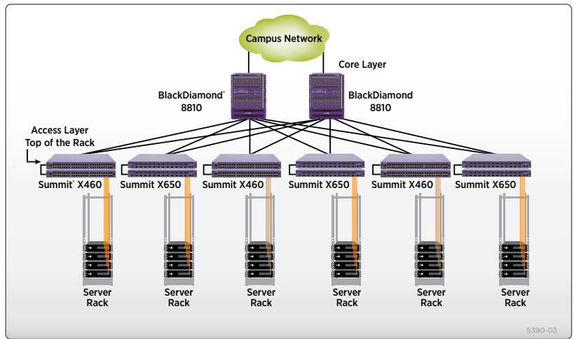
Figure 9: Top-of-Rack Architecture
