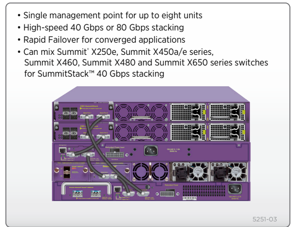
Figure 8: SummitStack Stacking Architecture
