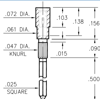
1045-3-17-XX-30-XX-02-0 Press-fit in .043 mounting hole
