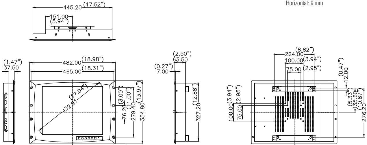
Cut out dimension 451 x 333 mm (17.75" x 13.38")
