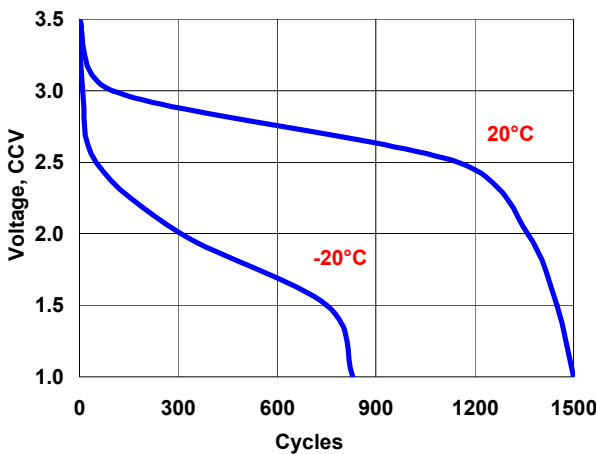
Typical Discharge Characteristics Schedule: 3 sec ON / 7 sec OFF Typical Drain: 1200 milliamperes
