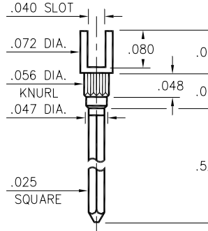
1122-0-23-XX-00-00-01-0 Press-fit in .053 mounting hole
