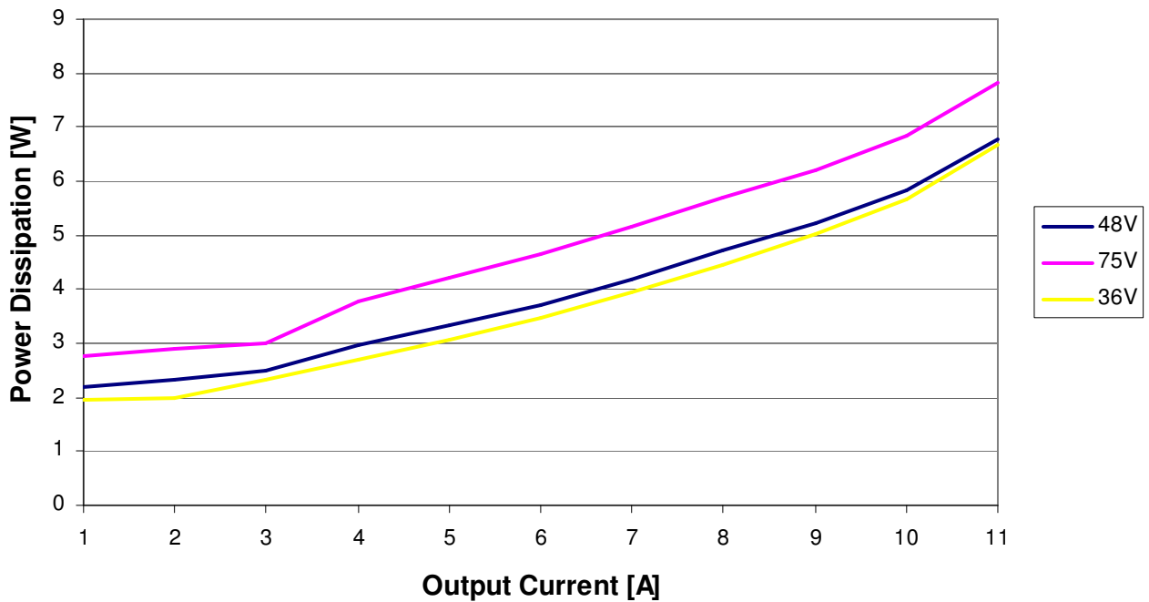
FIGURE 11: Power dissipation vs. load current for different input voltages at 25°C
