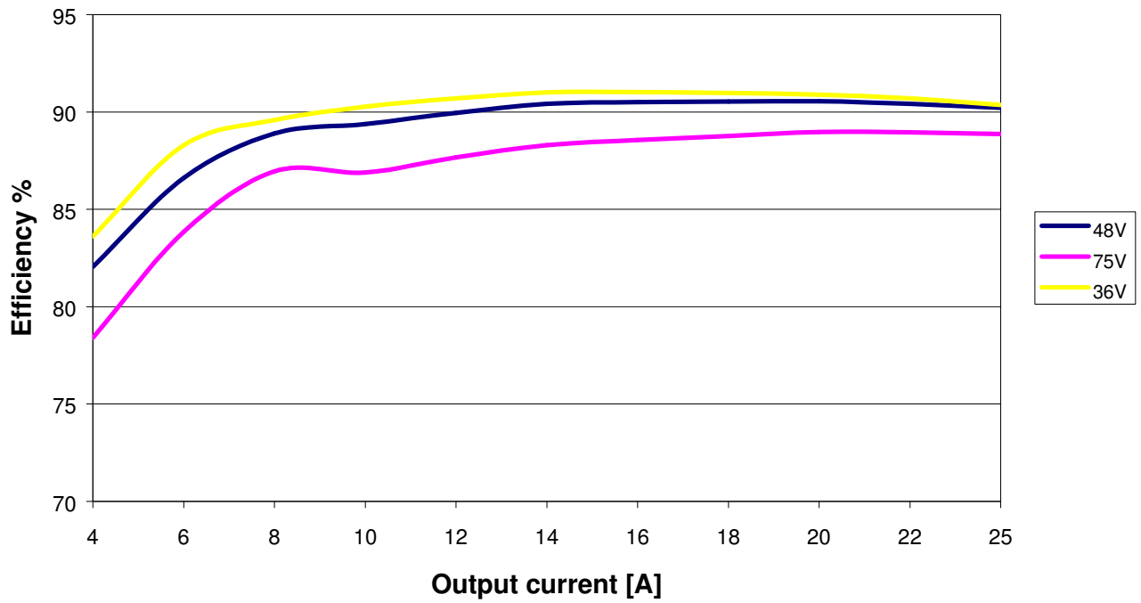
FIGURE 10: Efficiency vs. load current for different input voltages at 25°C
