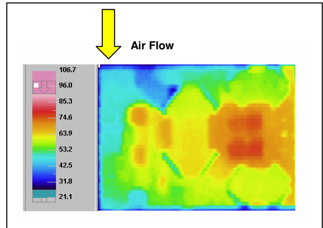
FIGURE 13: Thermal plot of converter: 25 A load, with 25°C air flowing at the rate of 200 LFM. Air is flowing across the converter from pin 1 to pin 3, at nominal input voltage.
