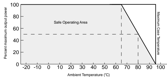
Fig. 24. Temperature Derating
