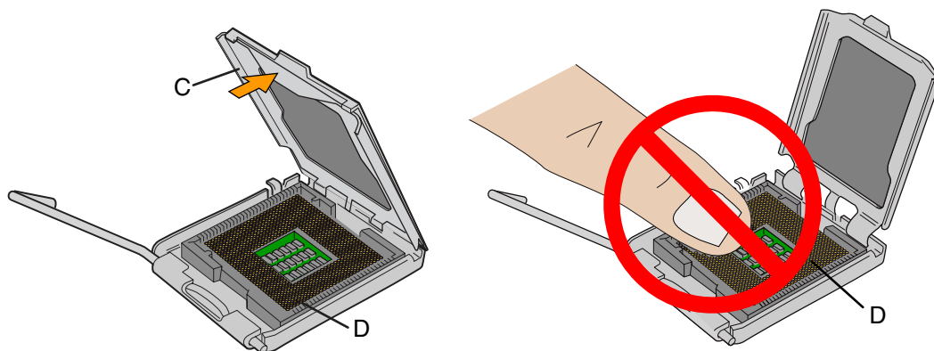
Figure 8. Lift the Load Plate and Don't Touch the Socket Contacts
