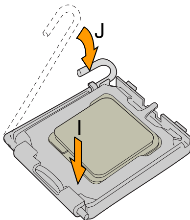
Figure 12. Close the Load Plate
