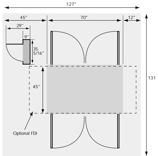
Concrete pad—suggested size
