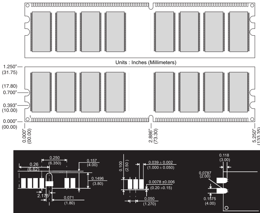
Figure 1: KVR266X64C25/1G 184-Pin DIMM
