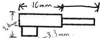
S.F.L. 90 DEG. LOW PROFILE COAX CONNECTOR
