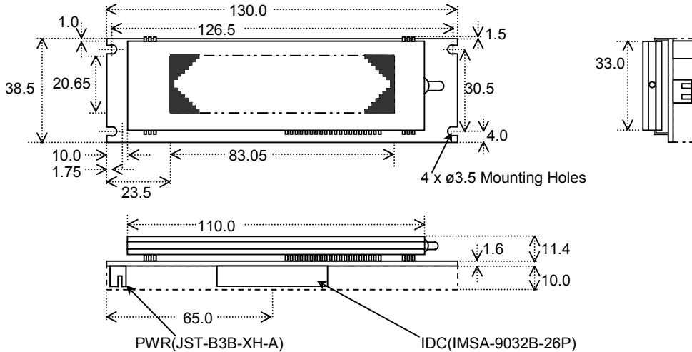
Dimensions in mm See full spec for tolerances
