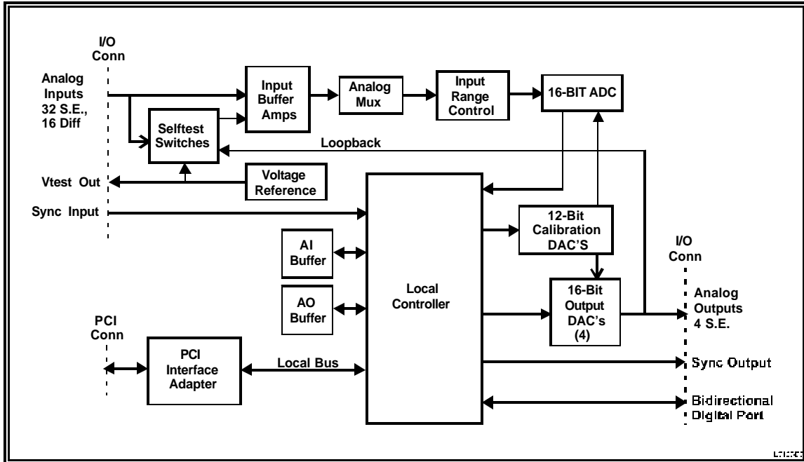
Figure 1. PCI-16AIO; Functional Organization
