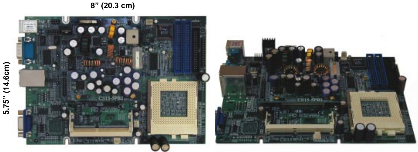
Photograph GCS15-SL above shows 1LAN, 1 PCI, and 12 VDC power
