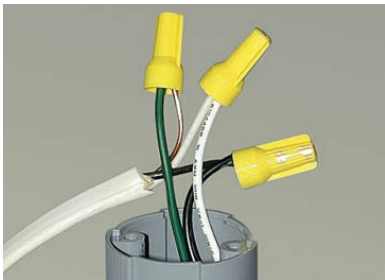
4. Connect receptacle wires to romex. Be sure to match wire color(s).
