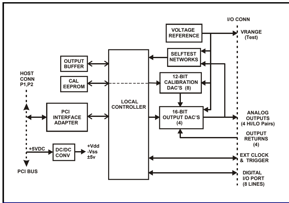
Figure 1. PMC-16AO4MF Board; Functional Organization
