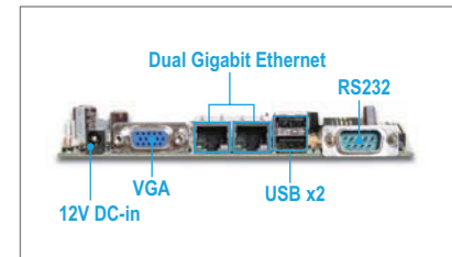
Rear I/O
